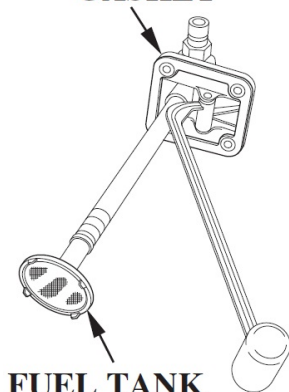
CONNECTOR GASKET
