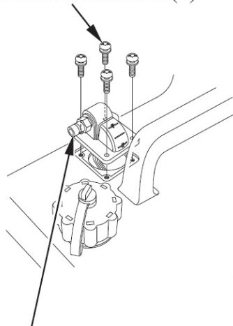
FUEL TANK FILTER JOINT (Fuel Hose Connector)
