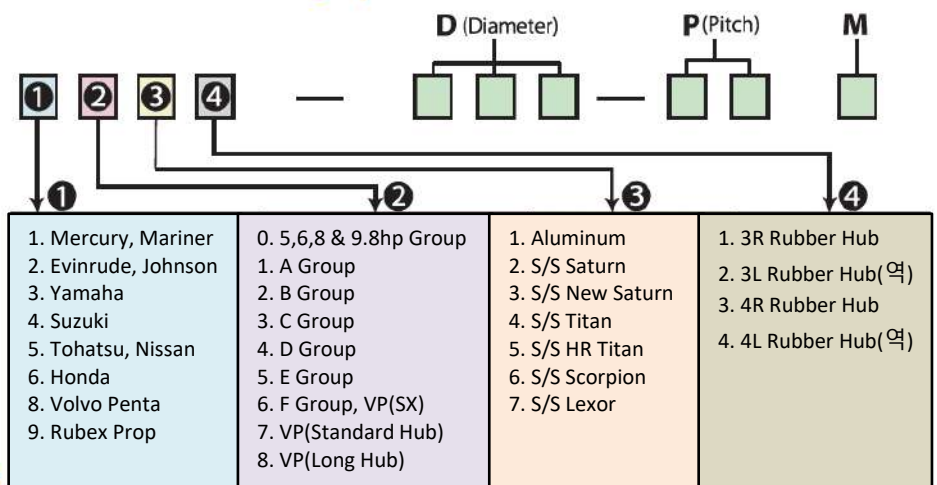
SOLAS Propeller Part No. on propeller.
